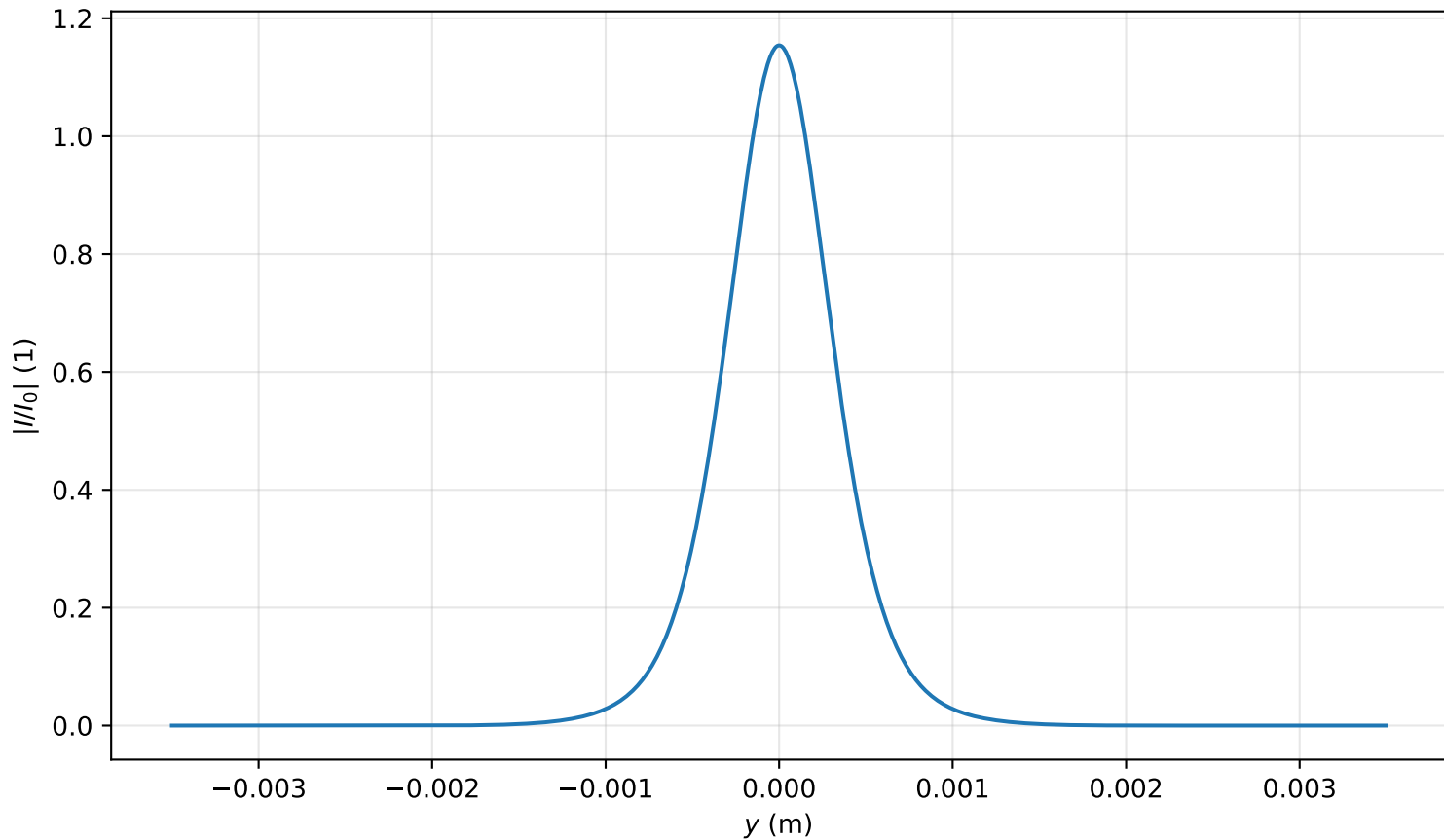
Intensity profile I(x=0, y, z=1.751)/I_0 , P_{in}=0.7P_{cr} , artificial time
